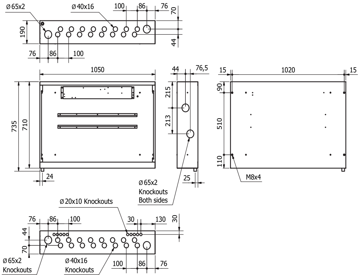
LK Manifold Cabinet Qmax 1050
