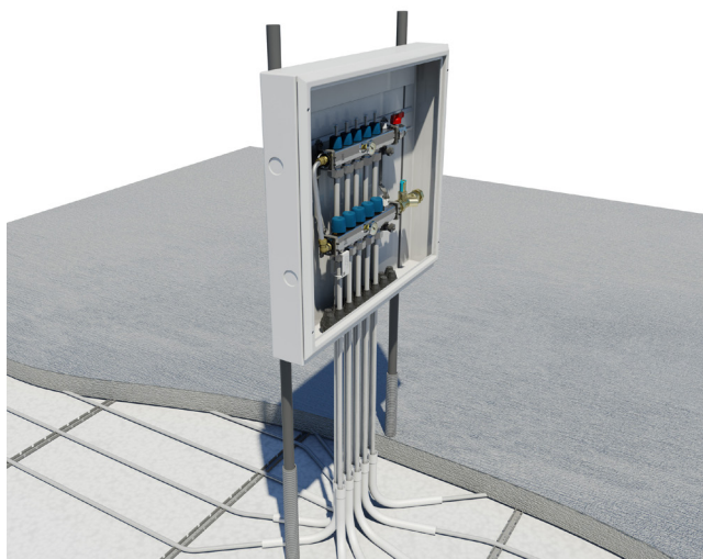
LK Cabinet Stand with LK Manifold Cabinet
