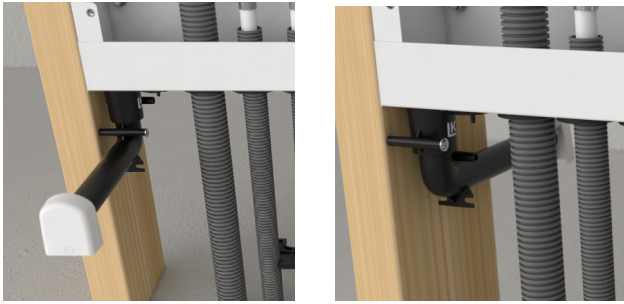
Illustration A drainage elbow directly connected to the cabinet's outlet pipe will drain into the same room as the cabinet's service hatch or, alternatively, the room behind.
