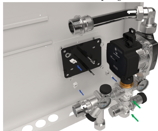
Installing the shunt bracket VS2.
