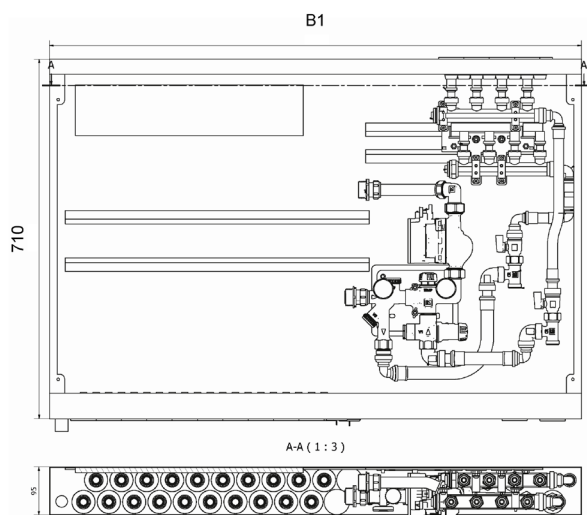
LK Combi Cabinet VS2 Prefab
