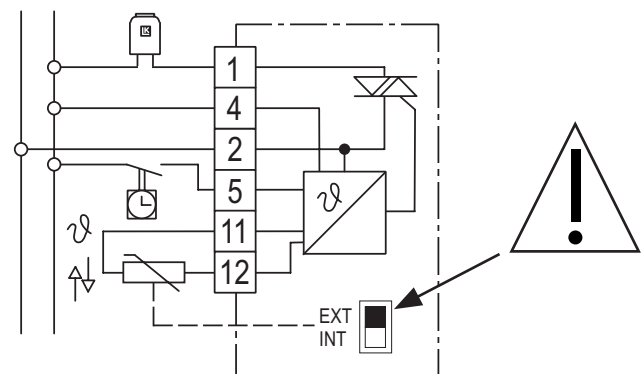
Circuit diagrams for LK Room Thermostat S1 EXT and LK Room Thermostat S1 Dti (The circuit diagram for LK Room Thermostat S1 is the same apart from the absence of terminals 11 and 12 for an external sensor)
