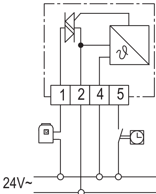
Connecting LK Room Thermostat S2
