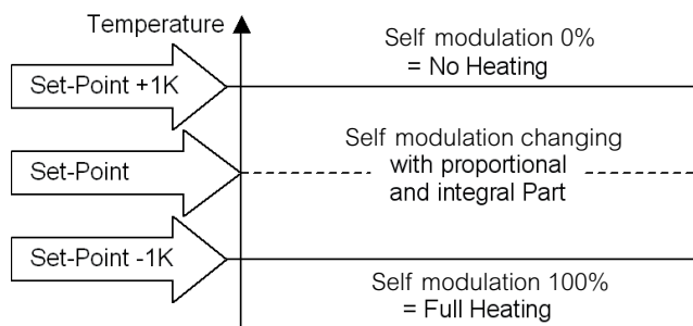
Temperature range for self-modulation, cycle time 42 min.
